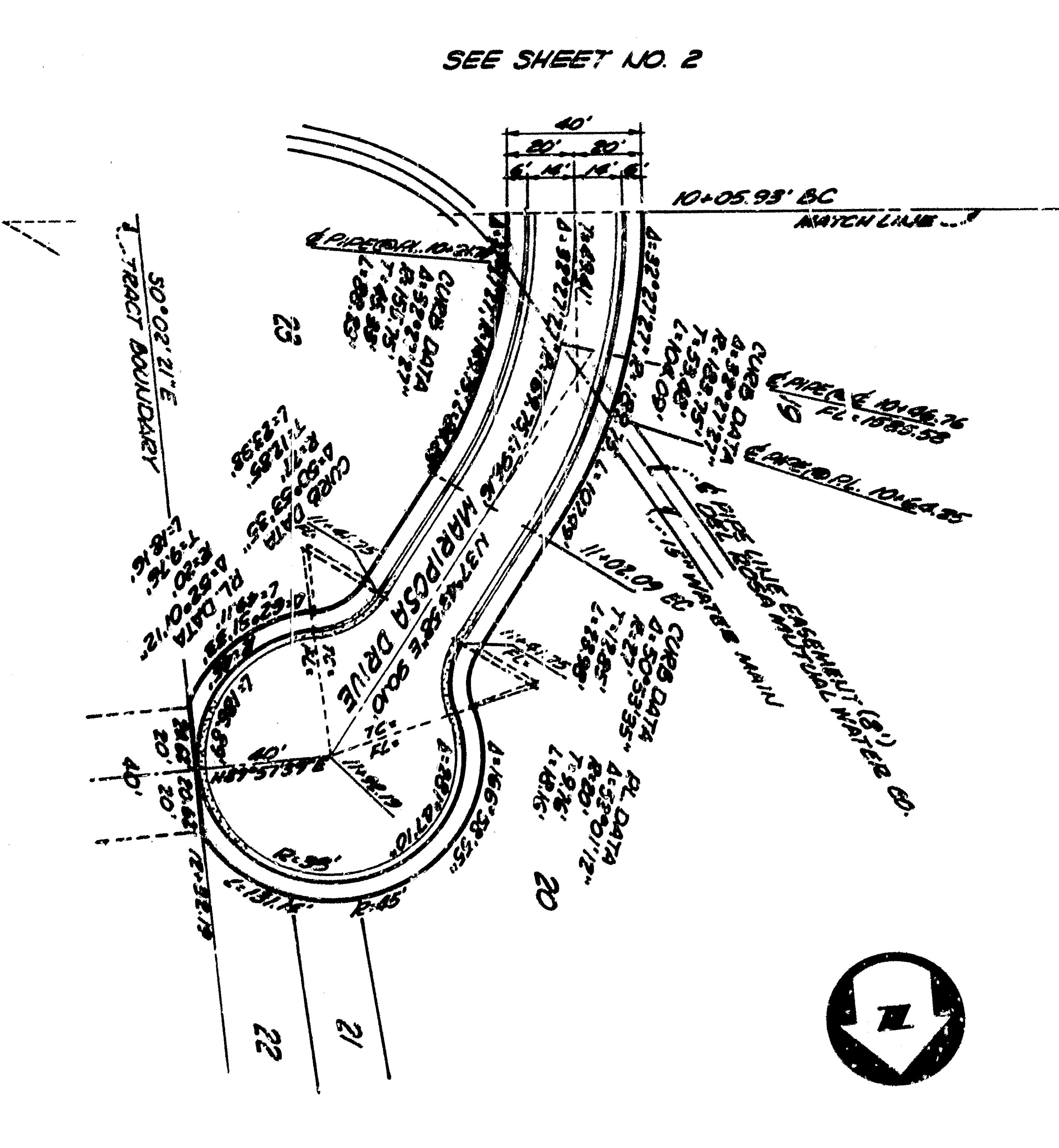
PLAN - MARIPOSA DRIVE SCALE: 1"=20'
